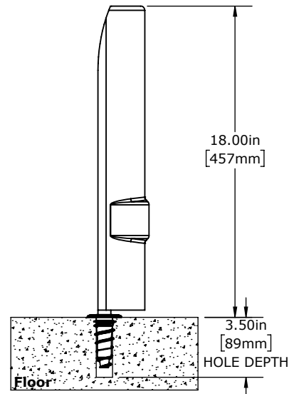
SIDE VIEW SCALE:1:8
