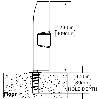
SIDE VIEW SCALE:1:8
